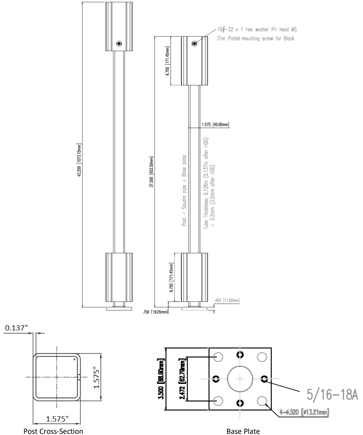
FIGURE 1 – ATLAS-PRO QUIK-MOUNT POSTS
