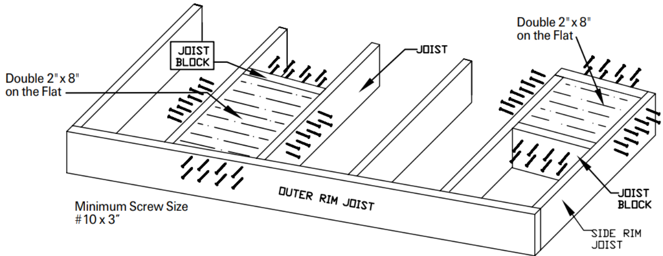
FIGURE 10 – BLOCKING DIAGRAM
